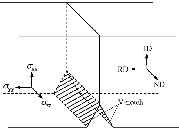
Fig. 10. Geometry of a notch and directions of the stresses. \sigma_{xx} , \sigma_{yy} and \sigma_{zz} : normal stresses in the x-, y- and z-directions, respectively. The direction of \sigma_{zz} is parallel to the notch front. The biaxial stress state at the free surface is plane stress ( \sigma_{zz} = 0 ).
