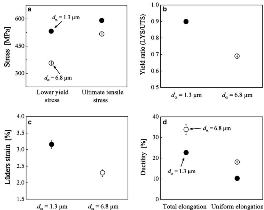
Fig. 3. Comparison of the tensile properties at room temperature of the steels with different ferrite grain sizes. The symbol d_\alpha refers to the average ferrite grain diameter. (a) strength; (b) yield ratio: lower yield stress/ultimate tensile stress (LYS/UTS); (c) Lüders strain; (d) ductility.
