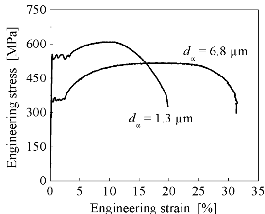
Fig. 2. Comparison of engineering stress-strain curves of the steels with different ferrite grain sizes. The different grain sizes were produced by the conventional route (without large strain warm deformation) and the ultrafine grain route, respectively. The ultrafine grain route involved a warm deformation procedure with four steps (each deformation step with \varepsilon = 0.4 and \dot{\varepsilon} = 10 \text{ s}^{-1} ) and a subsequent 2 h annealing treatment at 823 K. The symbol d_\alpha refers to the average ferrite grain diameter.
