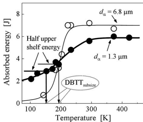
Fig. 4. Dependence of the Charpy impact properties on temperature of the steels with different ferrite grain sizes. The symbol d_\alpha refers to average ferrite grain diameter. DBTT subsize : ductile-to-brittle transition temperature of subsize specimen with a ligament size of 3 \times 4 \text{ mm}^2 . The ductile-to-brittle transition temperature was determined by using the correlations recommended in [31].
