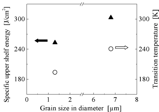
Fig. 7. Charpy impact properties of the steels with different ferrite grain sizes. The symbol d_z refers to average ferrite grain diameter. The specific upper shelf energy and the transition temperature in this context are the energy and temperature related to the ligament area for a full size specimen. These were converted from the results of subsize specimens by using the correlations recommended in [31].
