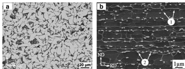
Fig. 1. (a) Light optical micrograph of the initial ferrite-pearlite microstructure of the steel processed by the conventional route (without large strain warm deformation). (b) SEM image of the ultrafine grained steel processed by the ultrafine grain route (with warm deformation, \varepsilon = 0.4 \times 4 , and subsequent 2 h annealing at 823 K). The white markers (number 1) highlight the dispersion of cementite particles inside the ferrite grains and the alignment of cementite particles along the ferrite grain boundaries (number 2).
