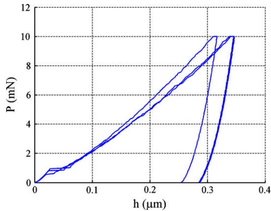
Fig. 4. Load–displacement curves for near-[101] indentation along [131 11]. The loading and unloading rates were both 2 mN/s, with a dwell time of 1 s. Initial Hertzian loading and subsequent pop-in is observed. One of the three curves was measured close to a grain boundary and greater hardening was observed in this case [90].
