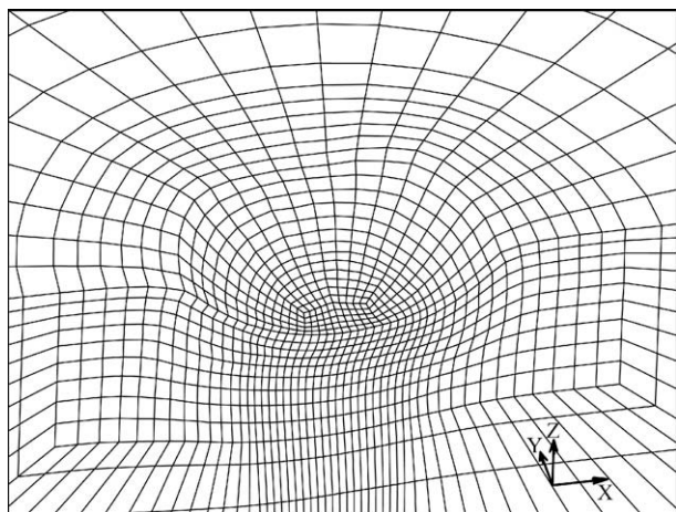
Fig. 2. A finite element mesh of 15,060 hexahedral elements after indentation; this was the maximum resolution of the indentation process, which was used for validation of the results with coarser meshes. Only half of the model is shown for better visibility of the mesh structure.
