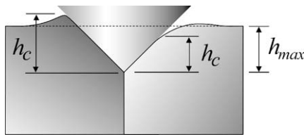
Fig. 1. Material pile-up (left) and sink-in (right) increases or decreases the contact height, h_c , during indentation to the maximum penetration depth, h_{max} .
