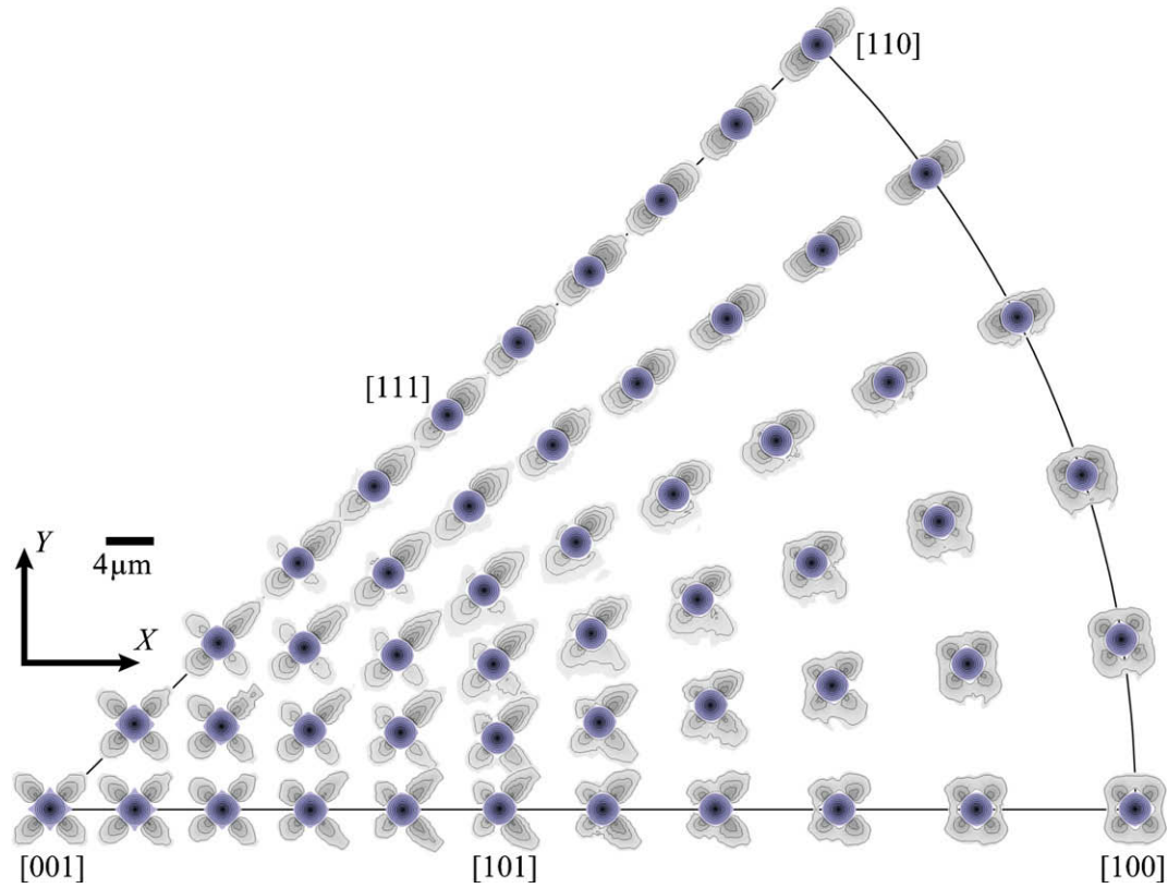
Fig. 8. Predicted pile-up patterns from axisymmetric indentation in \gamma -TiAl. The topographic data were obtained from 51 CP-FEM simulations; spherical tip with 146^\circ apex angle, tip radius 2.7 \mu\text{m} , maximum indentation depth 0.32 \mu\text{m} . The individual patterns are placed in an inverse pole figure (stereographic projection) of the respective indentation axes and in-plane oriented after the convention defined above, using the indicated indenter coordinates X and Y . The impressions are shown in bluish color (contour lines at -0.05, -0.1, -0.15 \mu\text{m} \dots ), the upheaval in greyscale (contour lines at 10, 20, 30 \text{ nm} \dots ). The number of dominant hillocks ranges from one, for an [111] indentation axis, to four, for axes [001] and [100] .
