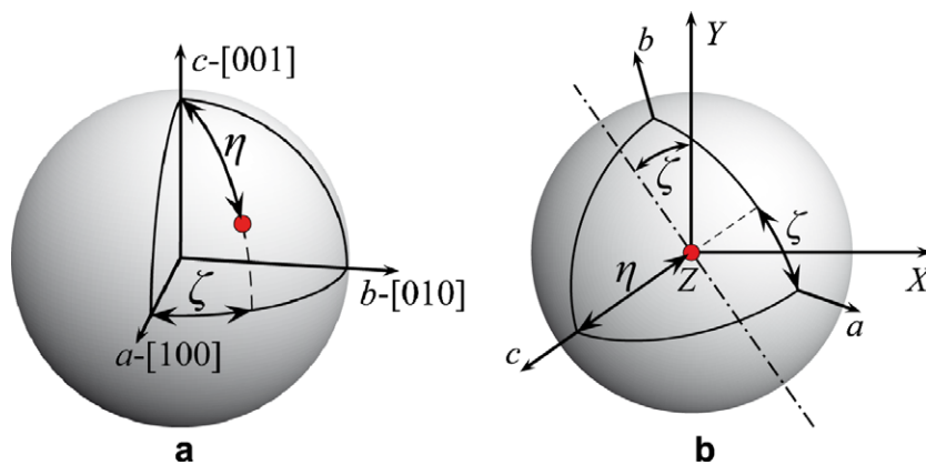
Fig. 7. Illustration of the orientation convention for displaying pile-up topographies. (a) The crystal coordinate system [x_c, y_c, z_c] , where x_c \parallel a, y_c \parallel b and z_c \parallel c ; a desired indentation direction, defined by the spherical coordinates (\zeta, \eta) = (35^\circ, 60^\circ) , is marked by the red dot. (b) The indenter coordinate system [X, Y, Z] , with the crystal rotated after the convention as defined in the text. Z is anti-parallel to the indentation direction. The rotation axis is shown by the dot-dash line.
