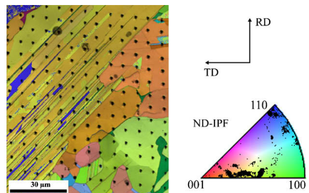
Fig. 3. A region with \gamma -grains in the nearly lamellar microstructure; the EBSD orientation map was acquired using the recently developed fit-rank indexing. The crystallographic orientation (in color) is overlaid with the image quality measure (in greyscale). Berkovich indents, made with a maximum load of 3 mN and arranged on a square grid with a nominal spacing of 6 \mu\text{m} , are visible through a reduced pattern quality. The inverse pole figure coloring scheme is also shown, with the measured orientations in black. Indentations with an axisymmetric indenter were applied in selected regions of the microstructure.
