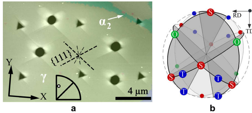
Fig. 5. (a) Nanoindentations in a \gamma -grain of nearly lamellar Ti-46Al-8Nb (at.%), shown by an AFM topographic map (greyscale) combined with an EBSD orientation map ([001] inverse pole figure coloring, cf. Fig. 3). The \{111\} -traces coincide with the observed surface steps. Sphero-conical (nominal tip radius R < 1 \mu\text{m} ) and Berkovich indentations were performed with maximum loads of 6 and 3 mN, respectively. Indentation axes were oriented along [1106] ; the X - Y coordinates are oriented after the convention that is defined in Section 4.2. (b) Illustration of the crystal orientation of the \gamma -phase in subfigure (a) (perspective projection): the \{111\} -planes are shown together with the shear directions for ordinary dislocation glide (O, green), superdislocation glide (S, red) and twinning (T, blue).
