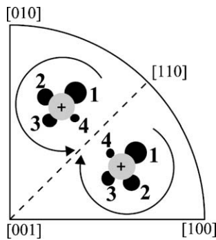
Fig. 6. The pile-up topography is changed under the influence of an improper symmetry operation; the developed surface profiles change their sense of rotation. The pile-up patterns of two indented orientations of \gamma -TiAl, connected by an improper symmetry operation, exhibit mirror symmetry through the (110) plane.
