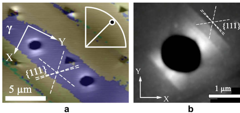
Fig. 9. (a) Topography (greyscale) of two sphero-conical indents in a coarse \gamma -phase lamella of orientation [14132] (cf. the inverse polefigure projection of the indentation axis); color indicates grain orientations. The greyscale shading ranges to about 18 \text{ nm} surface elevation. The maximum indentation load was 6 \text{ mN} . The inscribed X - Y coordinate system is in-plane rotated after the defined convention. Four Berkovich indentations (maximum load 3 \text{ mN} ) are also visible. (b) Higher resolution topography of one of these indents, in-plane rotated after the convention defined in Section 4.2.
