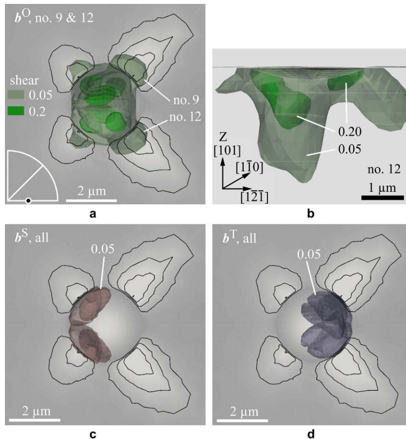
Fig. 11. Simulated surface topography from Fig. 10c, overlaid with the plastic shear distribution: (a) highly activated ordinary slip systems nos. 9 and 12, cf. Table 1, shown by semi-transparent isosurface levels at levels 0.05 and 0.2, differentiated by saturation; (b) shear on system no. 12, viewing the axis perpendicular to the shear direction [1\bar{1}0] ; (c) all superdislocation systems (red isosurfaces: shear level 0.05); and (d) all twinning systems (blue isosurfaces: shear level 0.05).
