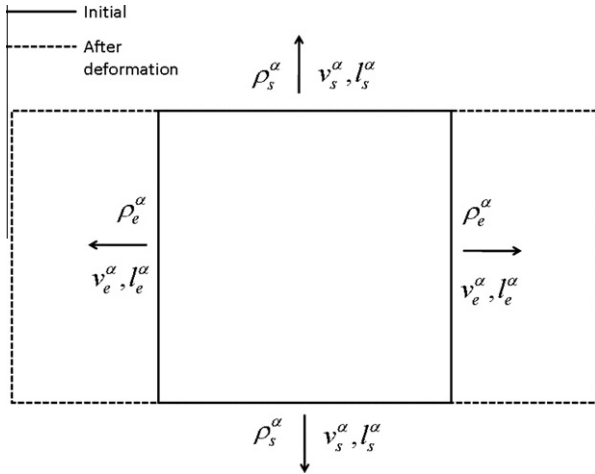
Fig. 4. Schematic of the expansion of a dislocation loop due to different velocities of edge and screw dislocation. \rho_x^\alpha , v_x^\alpha , l_x^\alpha represent the dislocation density, velocity, and segment length, respectively, for x type dislocations where x is edge or screw. i represents slip systems 1, 2 and 3, i.e. (\bar{1}010)[\bar{1}2\bar{1}0] , (1\bar{1}00)[\bar{1}\bar{1}20] and (01\bar{1}0)[2\bar{1}\bar{1}0] .
