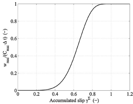
Fig. 9. Normalized nucleation probability w_{\text{nuc}}/(C_{\text{nuc}} \Delta t) against accumulated slip; the shape parameters are b=0.68 and c=6 .
