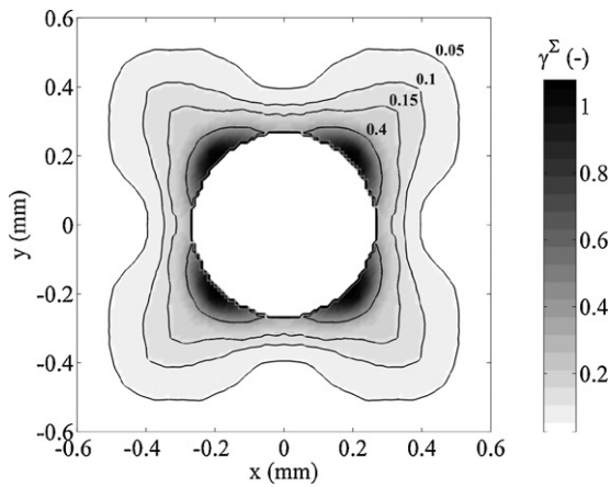
Fig. 8. Simulated profile of accumulated slip around an 1.47 kN indent, 10 \mu\text{m} below the initially undeformed sample surface plane. Contour lines are drawn at slip levels 0.05, 0.1, 0.15 and 0.4. The mark of the indenter has a diameter of 530 \mu\text{m} .
