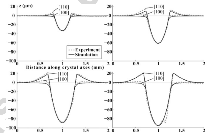
Fig. 6. Comparison of experimental and simulated topography of the indents. Each diagram depicts height profiles in the two directions [110] and [100]. Generally a pronounced pile-up is observed in the [110] direction. The height to width axes aspect ratio is 10:1.
