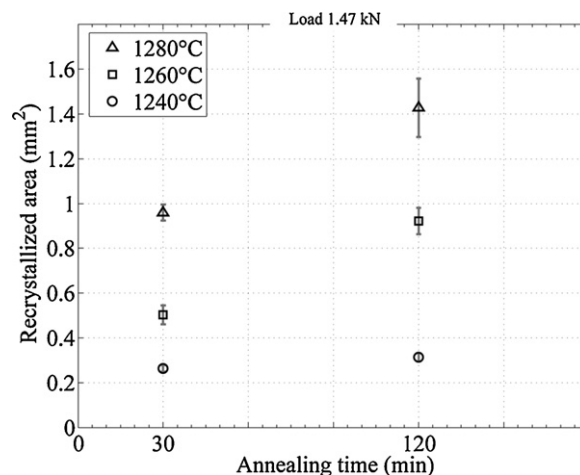
Fig. 3. Time and temperature dependence of the recrystallized area around an 1.47 kN indent in a (001) cross-section corresponding to the formerly undeformed surface. Also shown is the standard deviation calculated from the five measured values.
