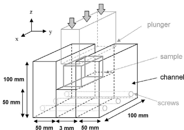
Fig. 1. Schematic drawing of the channel die plane strain set-up.
