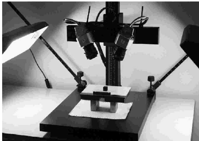
Fig. 3. Schematic drawing and photo of the experimental set-up of the CCD camera system.
