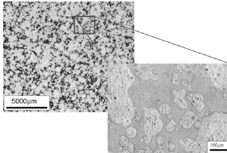
Fig. 2. Sprayed gray scale pattern on the surface of an undeformed polished and etched aluminum sample. The upper left picture was taken by digital optical microscopy. The lower right picture was taken in the scanning electron microscope. Images of this kind, taken before and after straining, were used for the photogrammetric calculation of the plastic displacement fields. For the spray, a color was chosen which did not affect the orientation measurement via electron backscattering diffraction.
