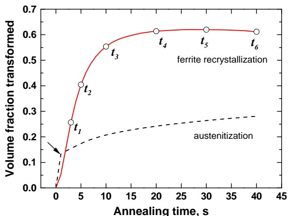
Fig. 4. Kinetics of ferrite recrystallization and austenite formation in the cold-rolled DP steel intercritically annealed at 760 °C. Here, a fast initial heating rate is imposed.
