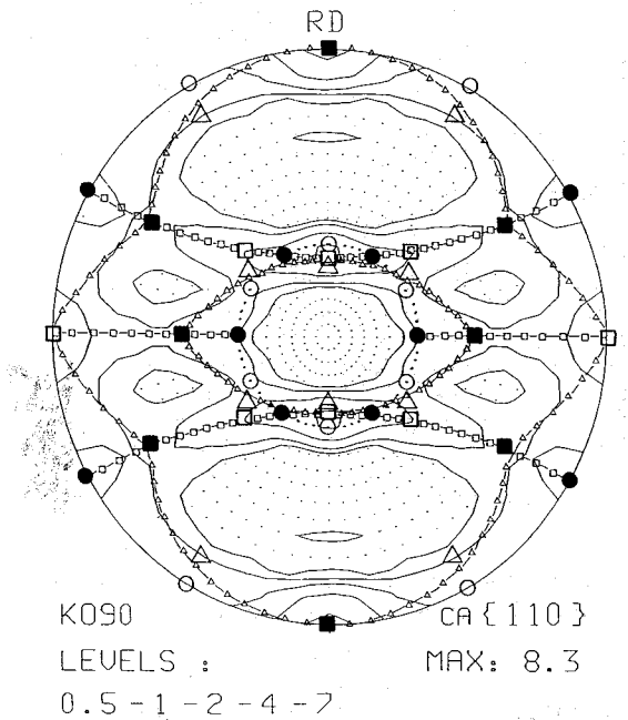
Figure 3. Fibres in a pole figure
