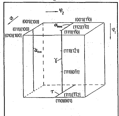
Fig.1 Definition of fibres in reduced Eulerspace
