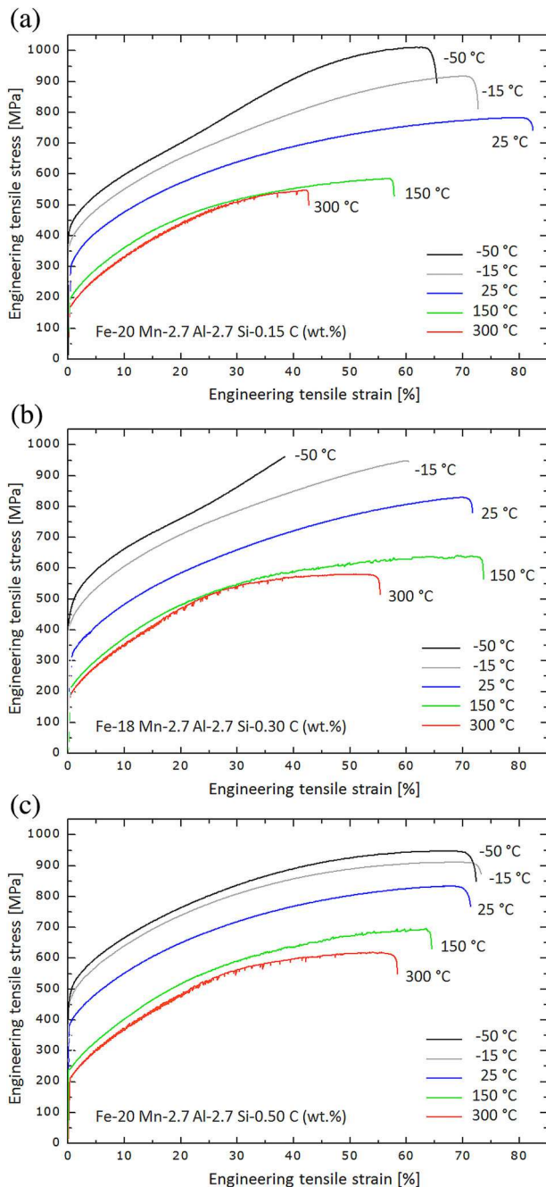
Figure 2. Stress–strain curves taken for quasi-static tensile tests conducted at different testing temperatures between -50 and 300 °C for high-entropy steels in the quinary system Fe–Mn–Al–Si–C. The trend toward deformation-induced martensite formation, resulting from different degrees in stability of the fcc solid solution phase at the onset of plastic straining, leads to different strain hardening characteristics (see also martensite characterization shown in Figure 3). Some of the curves are reproduced from earlier experiments conducted by the group of Frommeyer. [56–61,73,75] Of special relevance is the high ductility and high ultimate tensile strength observed at cryogenic temperatures of -50 °C. a) Fe–20Mn–2.7Al–2.7Si–0.15C (wt %); b) Fe–18Mn–2.7Al–2.7Si–0.30C (wt%); c) Fe–20Mn–2.7Al–2.7Si–0.50C (wt%). The experimental scatter was 1–4% for the ultimate tensile strength and 2–5% for the tensile elongation. The scatter was larger at higher temperatures.
