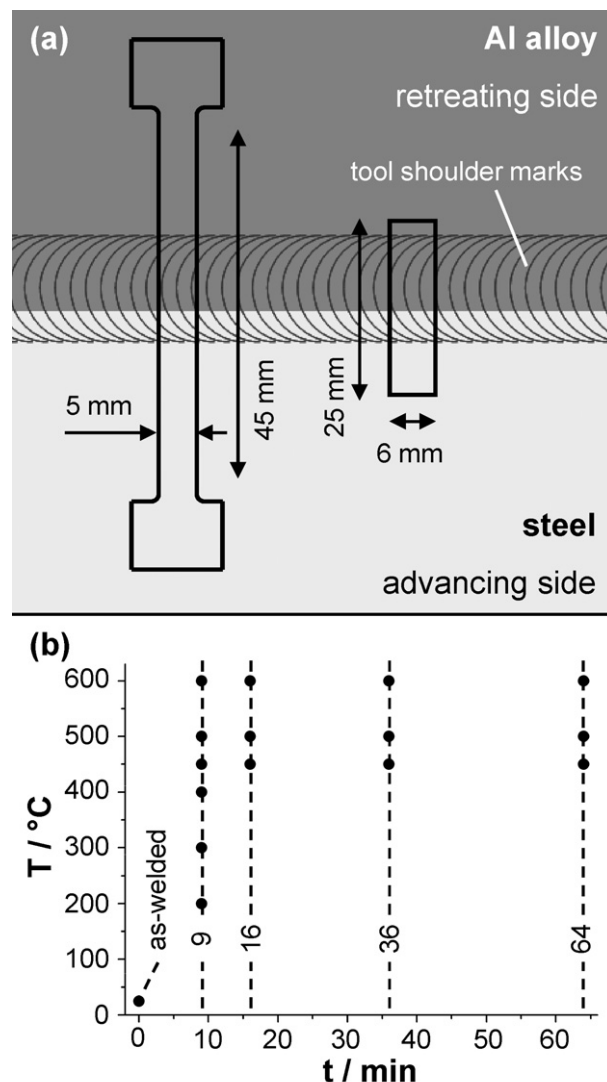
Fig. 1. Illustrations of the sample production process: (a) sketch of the friction-stir-welded base materials and the dimension and locations of samples for tensile testing (left) and interface characterisation (right). (b) Temperature/time matrix showing the different annealing treatments applied in this study.
