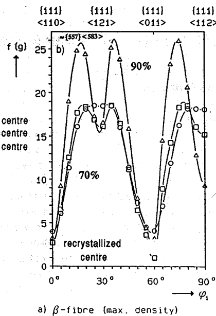
Figure 16a. Cold-rolling texture, center, Ti-microalloyed Fe-17%Cr steel
