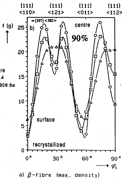
Figure 17a. Cold-rolling texture of a microalloyed Fe-17%Cr steel, \epsilon = 90\%
