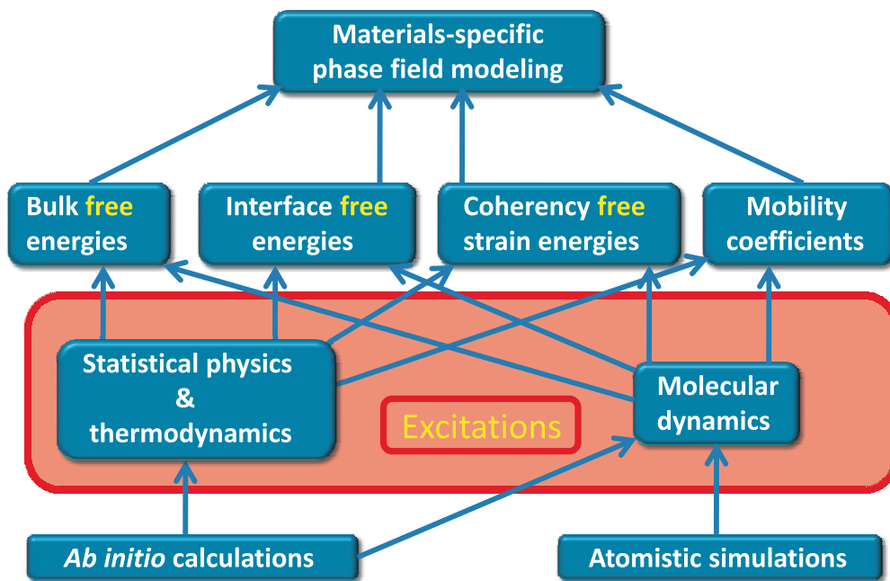
Fig. 11. Method-transfer of parameters within the multi-methodological scheme combining ab initio /atomistic calculations with the phase-field method.
