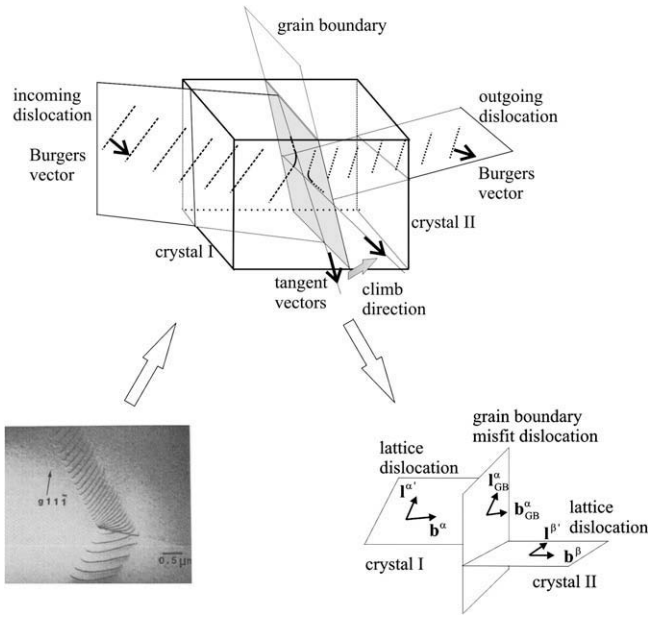
Fig. 9. Schematic drawing of penetration events for mobile dislocations through a grain boundary. The experimentally obtained micrograph is taken from the work of Shen et al. on steel [248]. Here l^a , l^b and l^a_{GB} are the tangent vectors of the dislocations, and b^a , b^b and b^a_{GB} are their Burgers vectors.
