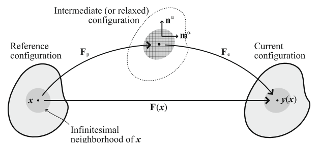
Fig. 5. Decomposition of the total deformation gradient, \mathbf{F} = \mathbf{F}_e \mathbf{F}_p .
