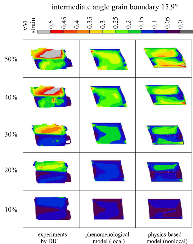
Fig. 33. Simple shear test of a bicrystal with a 15.9° intermediate-angle grain boundary (3.1 mm long, 2.0 mm thick and 2.2 mm high). Comparison of the von Mises strain patterns as obtained from the experiment via digital image correlation (DIC, left column), from the simulation with a conventional viscoplastic constitutive law (central column), and from the simulation which uses an advanced dislocation-based non-local model (see Section 4.3) (right column).
