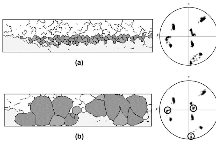
Fig. 38. Results of Bate from a network annealing model with the initial representation of microstructure derived from a CPFE simulation [155]. The initial number of crystallites was 900. Only grain boundaries with misorientations greater than 3^\circ are shown. Darker grains are near the cube orientation. The configuration at 400 remaining crystallites is shown in (b). The resulting grain orientations are given in the {001} pole figure [155].
