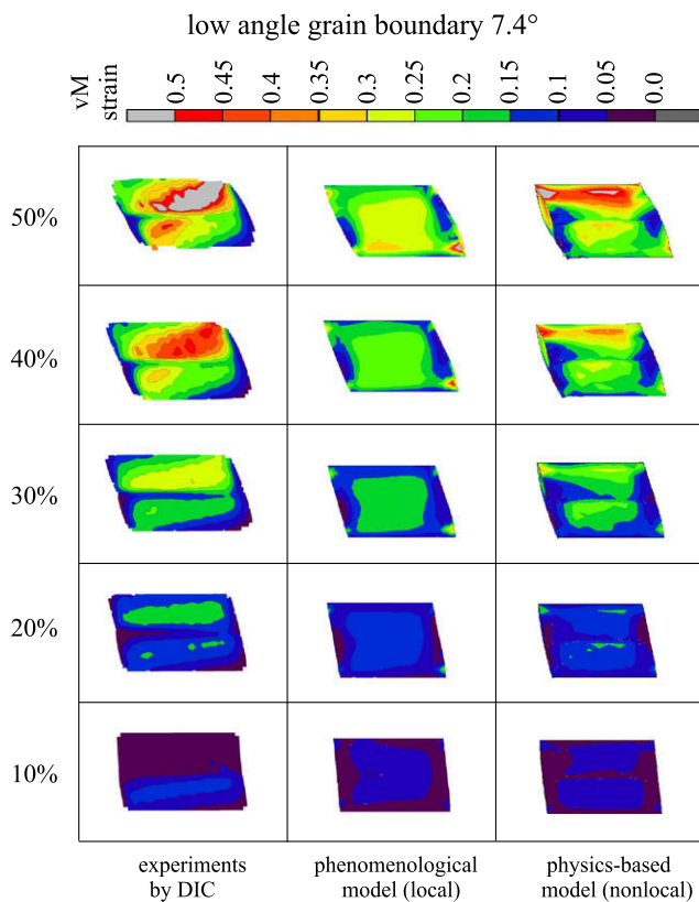
Fig. 32. Simple shear test of a bicrystal with a 7.4° low-angle grain boundary (3.1 mm long, 2.0 mm thick and 2.2 mm high). Comparison of the von Mises strain patterns as obtained from the experiment via digital image correlation (DIC, left column), from the simulation with a conventional viscoplastic constitutive law (central column), and from the simulation which uses an advanced dislocation-based non-local model (see Section 4.3) (right column).
