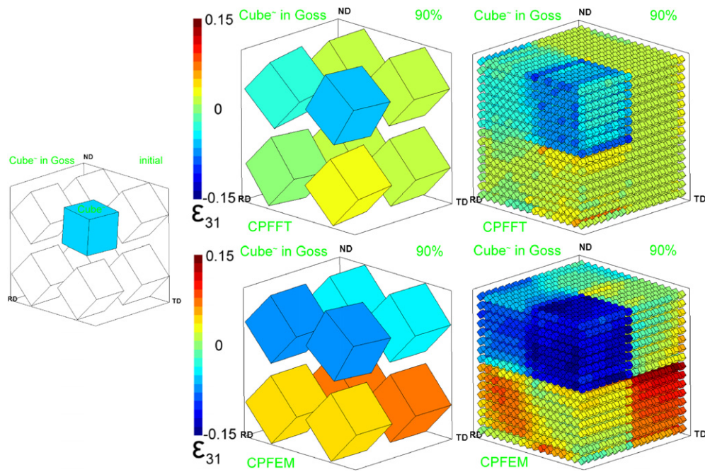
Figure 11. Final crystallographic orientations and strain states on the material points after plane-strain compression of a bicrystal (Cube~ in Goss) at 90% thickness reduction. The cube symbols are rotated according to the final orientations, and colored according to the values of strain component \epsilon_{31} . The results presented here are from the simulations run at the lowest resolution (1 Fourier point or element in the Cube~ grain and 1 \times 7 Fourier points or elements in the Goss grain) (left) and at the highest resolution (512 Fourier points or elements in the Cube~ grain and 512 \times 7 Fourier points or elements in the Goss grain) (right).
