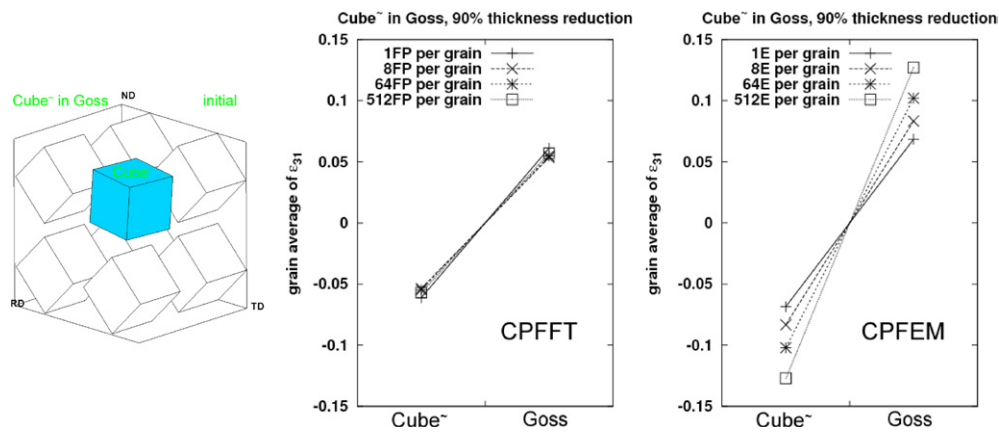
Figure 12. Plane-strain compression of a bicrystal (Cube~ in Goss) at 90% thickness reduction. The grain averages of strain component \epsilon_{31} are plotted considering the different volume fractions of the crystals (for the Cube~ grain \epsilon_{31} \times 1 , for the Goss grain \epsilon_{31} \times 7 ) for simulations run at different resolutions: 1, 8, 64, 512 Fourier points or elements in the Cube~ grain and 1 \times 7 , 8 \times 7 , 64 \times 7 , 512 \times 7 Fourier points or elements in the Goss grain.
