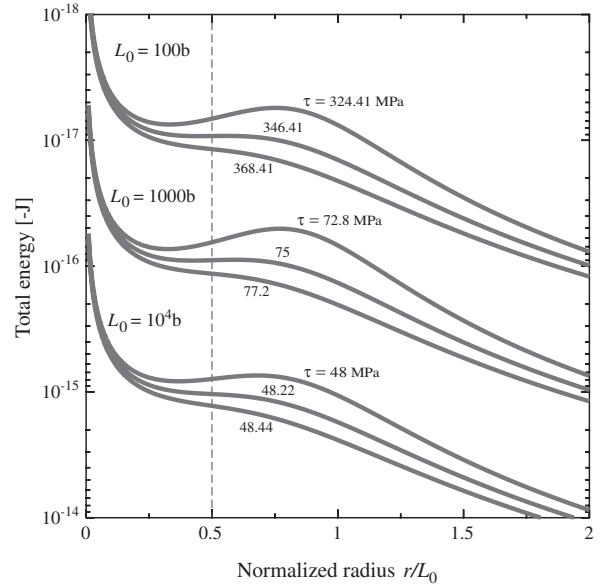
Fig. 3. Total energy ( Q_{\text{total}} ) of the twin nucleus. The numbers above each of the curves represent the applied shear stress. L_0 is the length of the sessile partial dislocations forming the twin nucleus and r is the distance the mobile partial dislocations have bowed out. An r/L_0 ratio of 0.5 is the critical ratio needed to be overcome in order for the twin to fully form. Less applied shear stress is required to form a twin as the size of the twin nucleus grows.
