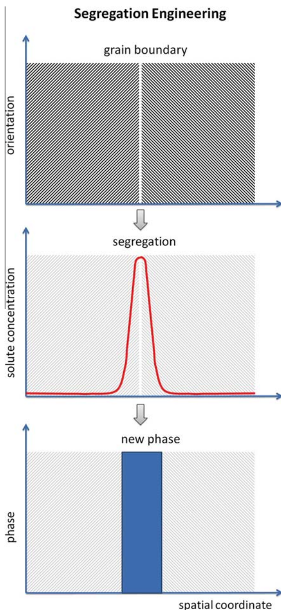
Fig. 1. Principle of “segregation engineering”. The approach is based on grain boundary segregation followed by nanoscale phase transformation of the decorated grain boundary region. Here we use Mn segregation to martensite grain boundaries followed by segregation-assisted and distortion-assisted martensite to austenite reversion at these grain boundaries.
