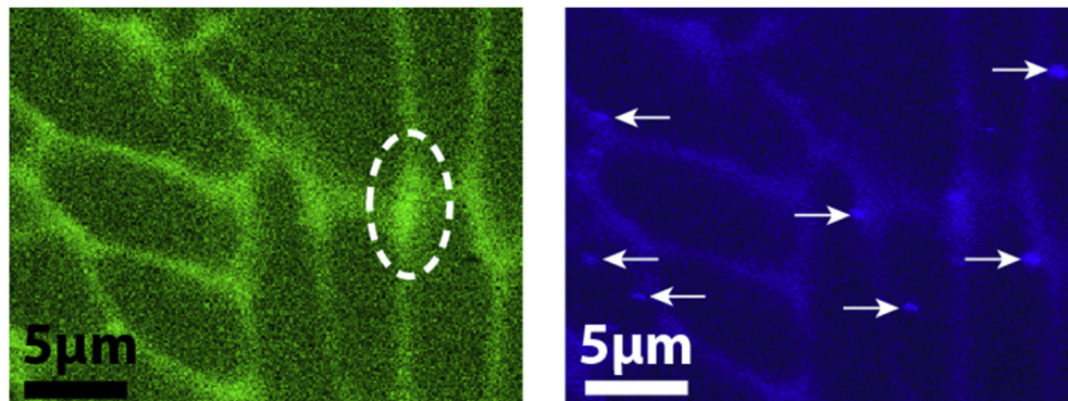
Fig. 3. EDS mappings from layer number 4 containing approximately 10 at% Al performed in the SEM showing Ni and Al enrichment at the dendrite boundaries. The Al rich dots observed in the Al map (marked by white arrows) were identified as Aluminum oxide particles. For both, Ni and Al, the K\alpha line was used for collecting the map signals.
