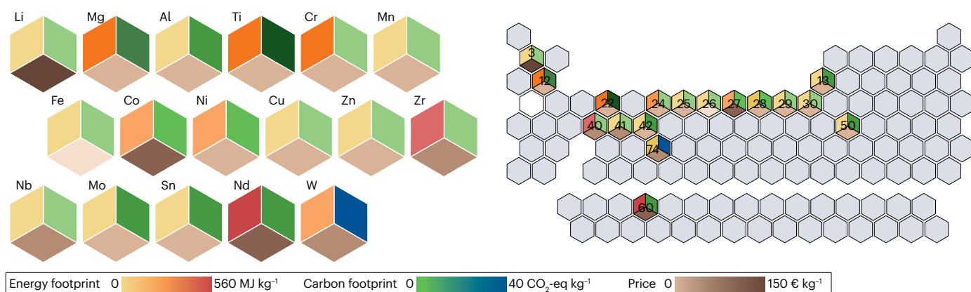
Fig. 6 | Sustainability and cost considerations for high-entropy materials.
