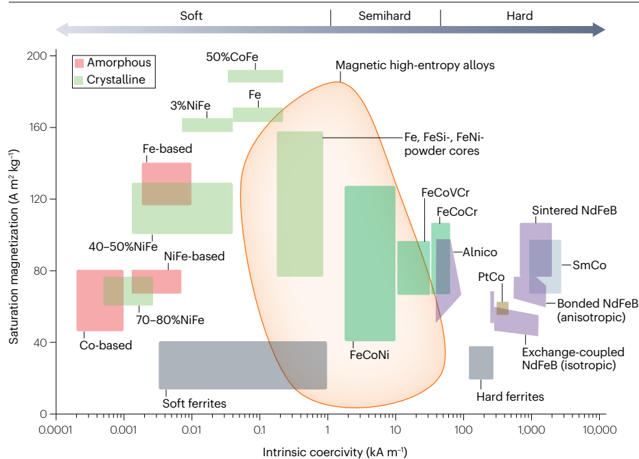
Fig. 4 | Magnetic properties of high-entropy materials. Saturation magnetization versus coercivity for several magnetic high-entropy materials (HEMs) compared with values for various soft and hard magnetic materials. Adapted with permission from ref. 260, Wiley.
