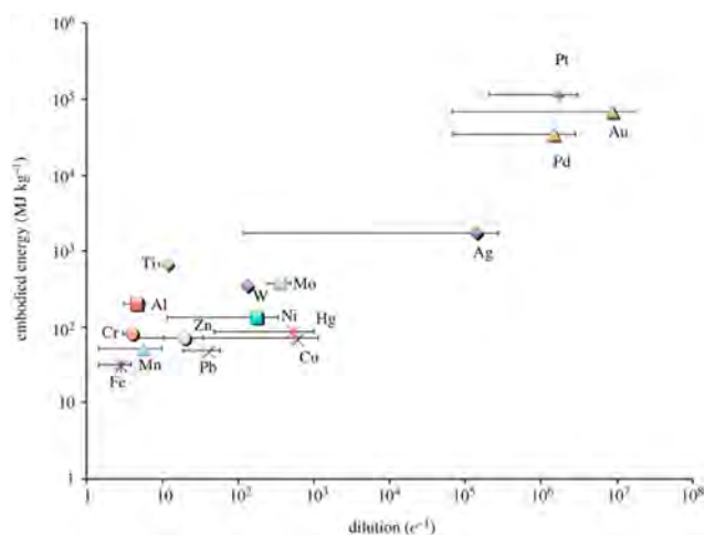
Figure 71. Relationship between dilution and embodied energy. 17 Figure is reproduced in modified form with permission from ref 17. Copyright 2013, The Royal Society.
