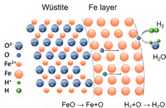
Figure 124. Some of the transport and redox processes involved during hydrogen-based direct reduction, where after the first surface reduction step a thin iron layer forms so that the oxygen must diffuse either through this solid material or through cracks and other defects that form due to the volume mismatch between the two phases (iron and oxide). 241 See also Figure 84, Figure 85, and Figure 123. The figure is reproduced in modified form with permission from ref 241. Copyright 2021, Elsevier.
