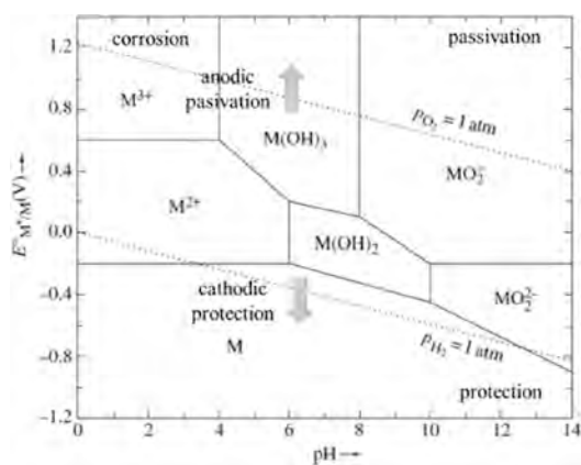
Figure 66. Pourbaix diagram showing regions of phase stability ranges of metals and metal oxides in water as a function of pH and reduction potential.
