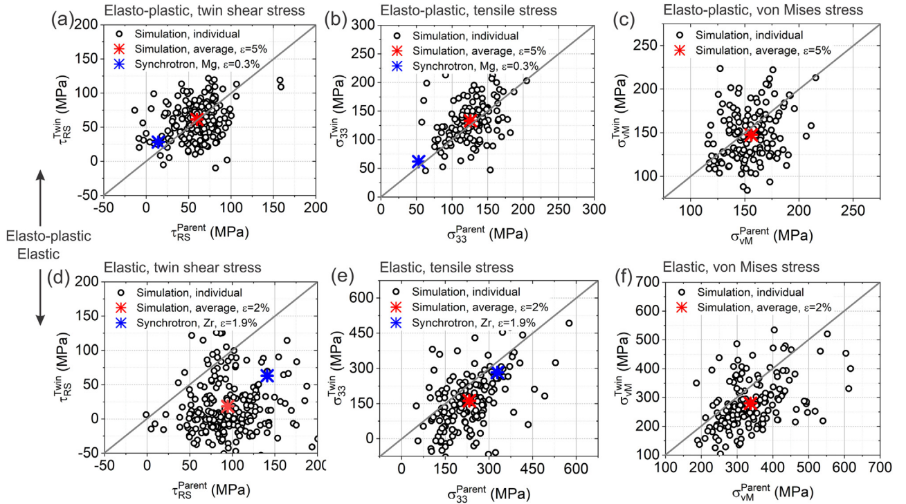
Fig. 8. Stress in the twin as a function of stress in the corresponding parent. Twin resolved shear stress (a), tensile stress (b), and von Mises stress (c) at a strain of 5%. (d–f) showing the results without considering dislocation accommodation at a strain of 2%. The asterisk symbols represents the average value for each population. The experimental results on an AZ31 Mg alloy [84] and pure Zr [85] measured by three-dimensional synchrotron X-ray diffraction are also included. The comparison and assessment of the simulations and experiments is presented in Section 4.1.
