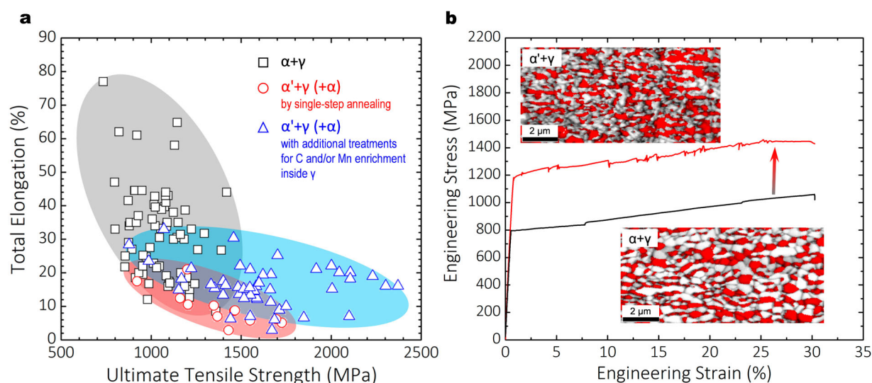
Figure 22. (a) Strength-ductility combinations of MMnS with different types of microstructure (plotted based on published data [1,8,14,16,18,42,47,68,141,151,192,229,233–245]); (b) Tensile behaviour of a 0.18C-8Mn (wt-%) steel fabricated to have either an austenite-ferrite microstructure (lower curve) and austenite-martensite microstructure (upper curve) with a similar austenite fraction ( \sim 44\% ); the austenite in the latter type of microstructure was stabilized by specially designed heat treatments for enabling sufficiently high-Mn and C enrichment. (b) is reconstructed with permission from Ref. [18].
