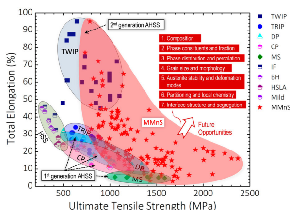
Figure 25. Comparison of tensile properties between MMnS and typical first/second-generation AHSS (plotted based on published data [1,8,14,16,18,26,42,47,68,141,151,192,229,233–245,253–262]). HSS: conventional high-strength steels, IF: interstitial-free steels, BH: bake hardenable steels, HSLA: high-strength low-alloy steels, Mild: mild steels, DP: dual-phase steels, CP: complex phase steels, MS: martensitic steels, TRIP: transformation-induced plasticity steels, TWIP: twinning-induced plasticity steels.
